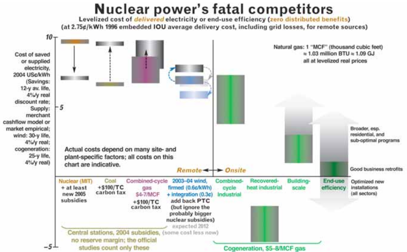
Fig. 3. The canonical 2003 MIT study, whose results continue to look conservative, says a new nuclear plant would produce electricity for about 7.0¢/kWh (2004 $). Adding the cost of delivery to the customers (at least 2.75¢/kWh) raises this busbar cost to 9.8¢ per delivered kWh. The decentralized competitors' delivered costs shown are those typically observed for well-executed projects in the U.S. marketplace, using assumptions that systematically favor nuclear power.
